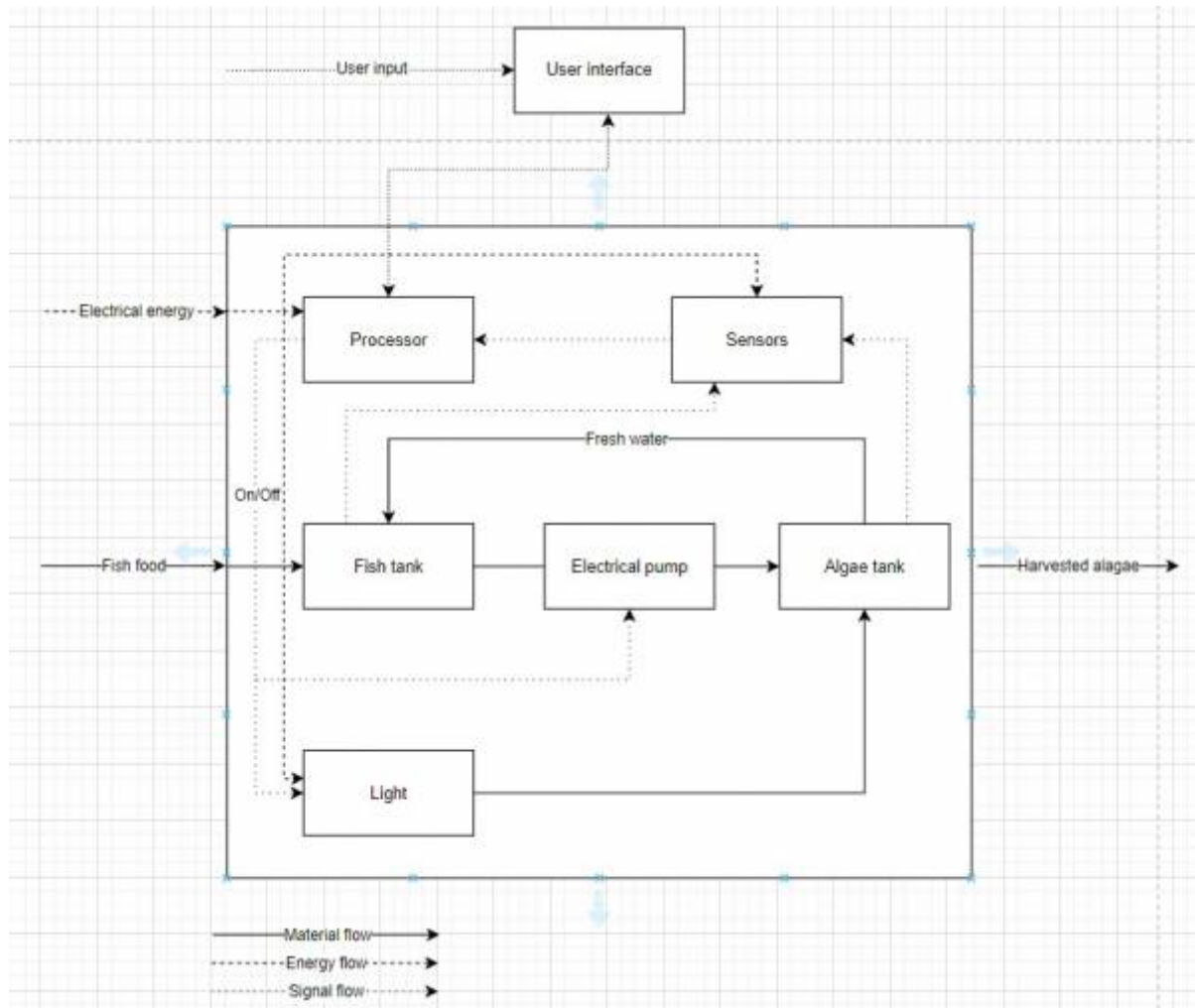
Figure 16: Black Box Diagram
