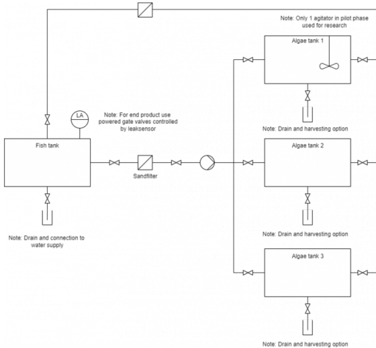
Figure 22: System Schematics Proposition
